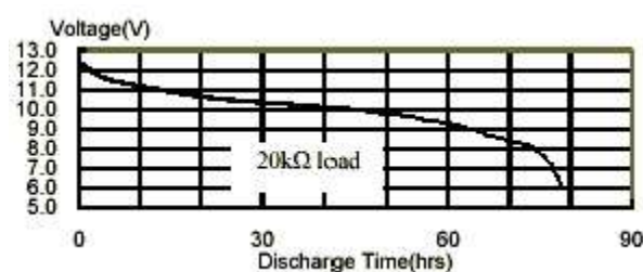
Typical Discharge characteristics at 20 ± 2 °C
